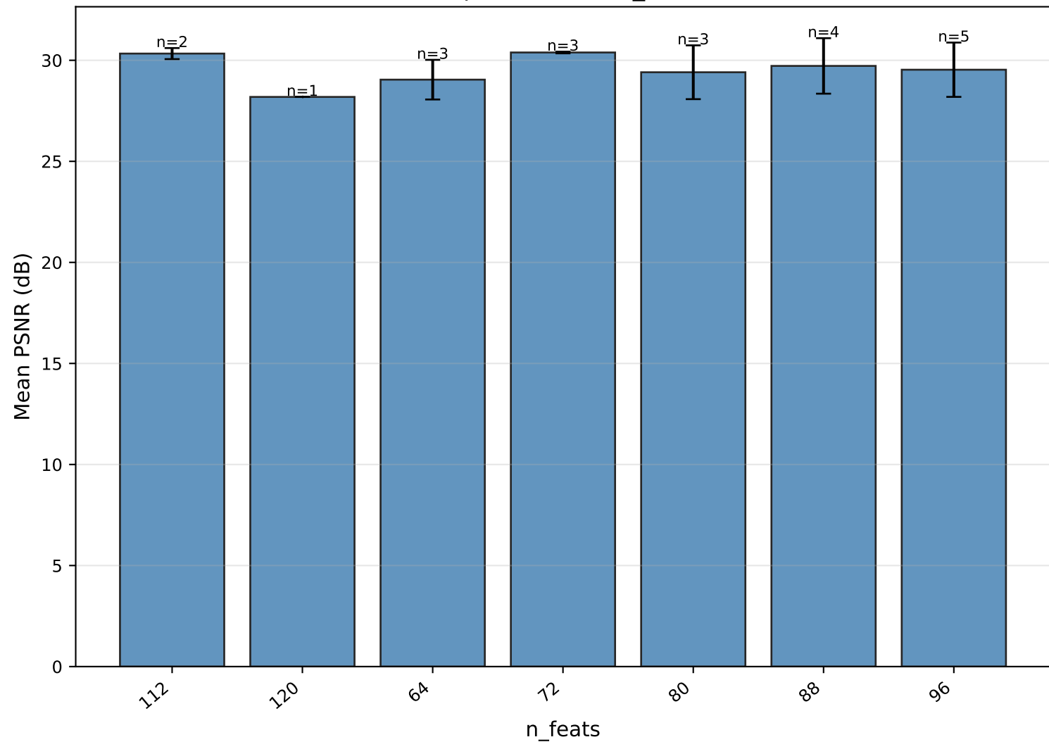
Mean PSNR per value of n_feats — ELAN
